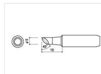
900L-T-5CF Shape-5C Tinned cut surface only
