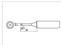
900L-T-2CF Shape-2C Tinned cut surface only
