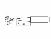
900L-T-2.4D Shape-2.4D
