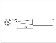
900L-T-2B Shape-2B
