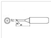
900L-T-2C Shape-2C
