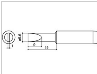
900L-T-S1 Shape-5.6D
