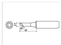
900L-T-4CF Shape-4C Tinned cut surface only
