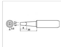
900L-T-3.2D Shape-3.2D
