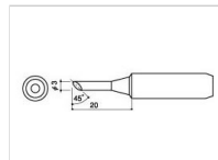
900L-T-3CF Shape-3C Tinned cut surface only
