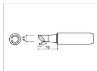
900L-T-5C Shape-5C
