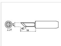
900L-T-K Shape-K
